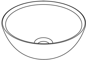
S32T Soft32 Table top washbasin 320 mm x 320 mm x 130 mm Height after installation 127 mm
