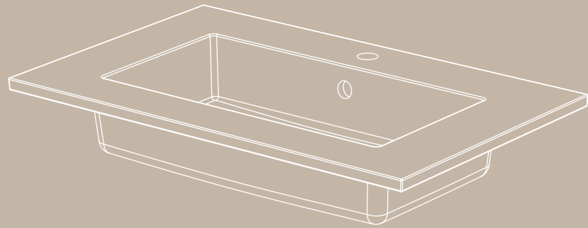
UNIT80 INTEGRATED 812 mm x 503 mm x 138 mm / Height after installation 20 mm EN 14688 – CL 10
